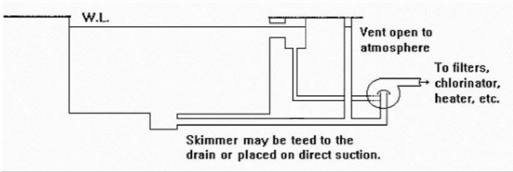
Figure 5. Vent System to Relieve Main Drain Suction B.5 Assessment of Gravity
